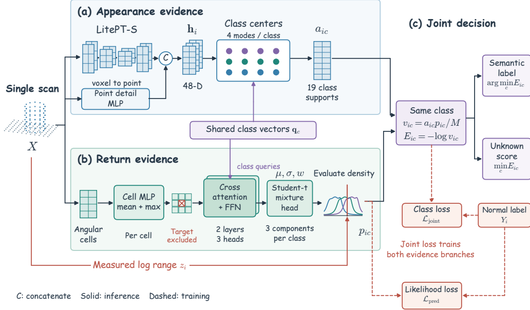
Figure 1: SERVE architecture. The full-scan branch combines voxel features with point details and projects them to a 48-dimensional embedding. Shared class vectors organize appearance centers and query independently encoded surrounding cells. Within the prediction branch, target exclusion precedes cross-cell attention; the actual target range enters only the subsequent density evaluation. Evidence combines within each class before semantic labeling and unknown scoring. Dashed paths show the joint classification and predictive likelihood objectives; auxiliary losses are specified in Equation (11). Point-cloud and density glyphs are schematic.
