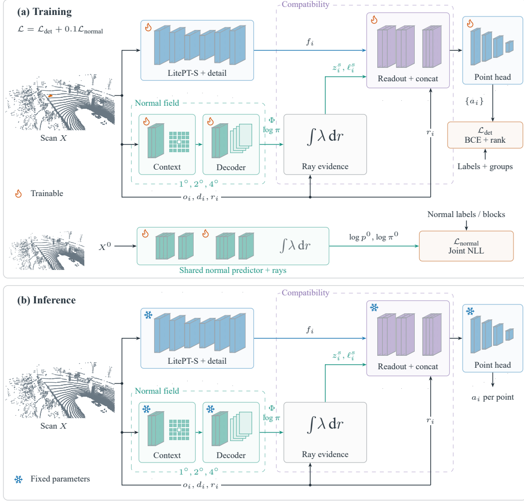
Figure 1: Contextual normal return fields. (a) Detection and original-scan likelihood jointly train the model. (b) Inference outputs one anomaly score per point. Ray evidence computes hypothesis log densities and marginal log density \ell_i^s , bundling densities with decoder log priors as z_i^s . Readout includes query formation, hypothesis attention and feature concatenation. The auxiliary path shares the normal predictor. Arrows show forward data dependencies; dashed boxes group computations. Flames mark trainable modules; snowflakes mark fixed inference parameters. Gray operators are analytic. Layer glyphs are schematic. The real nuScenes scenes share a viewpoint; orange marks auxiliary labels.
