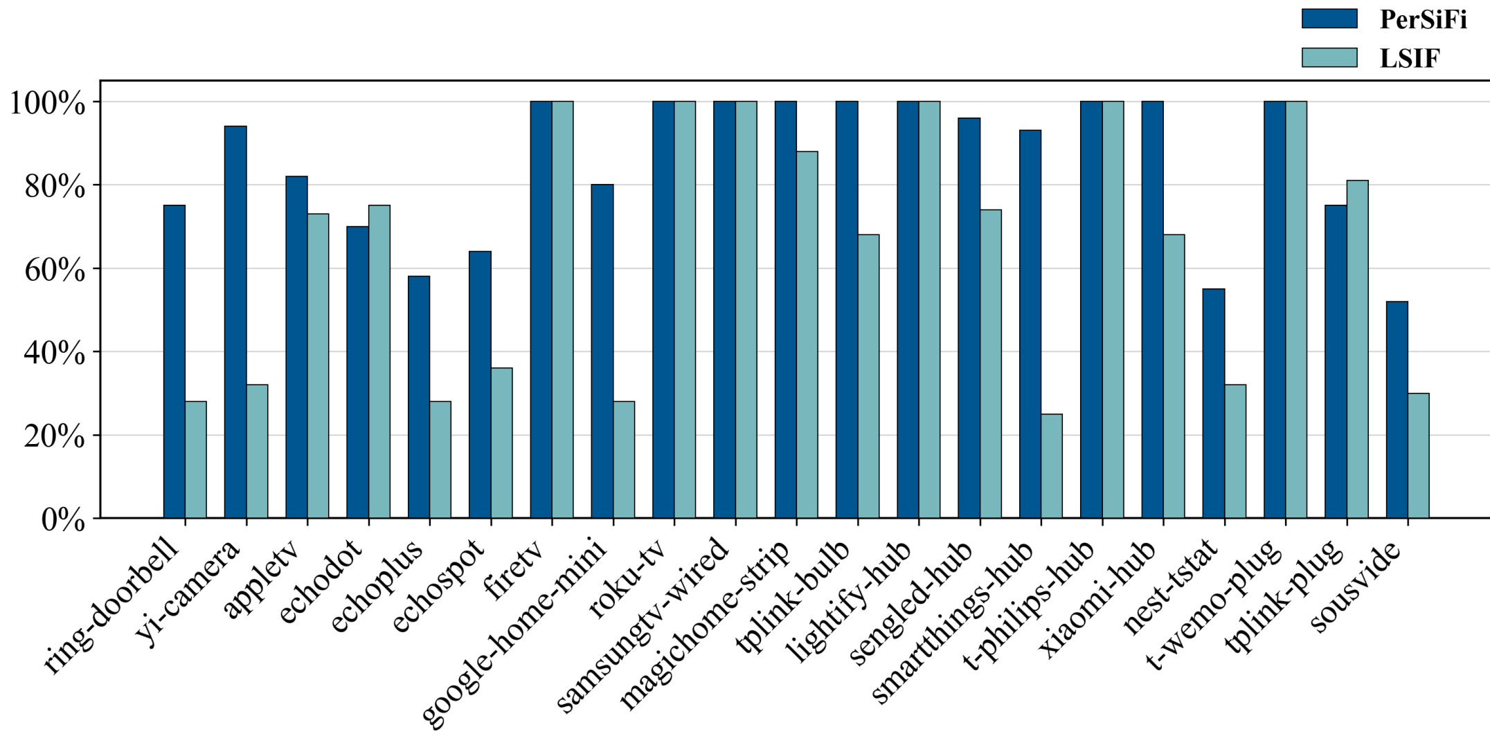
F1-score
