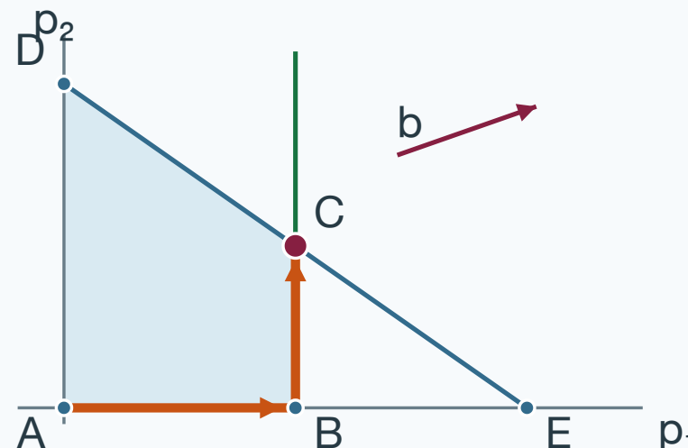
Dual variables
