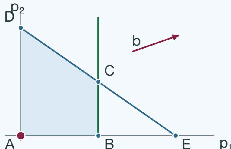
Dual variables
