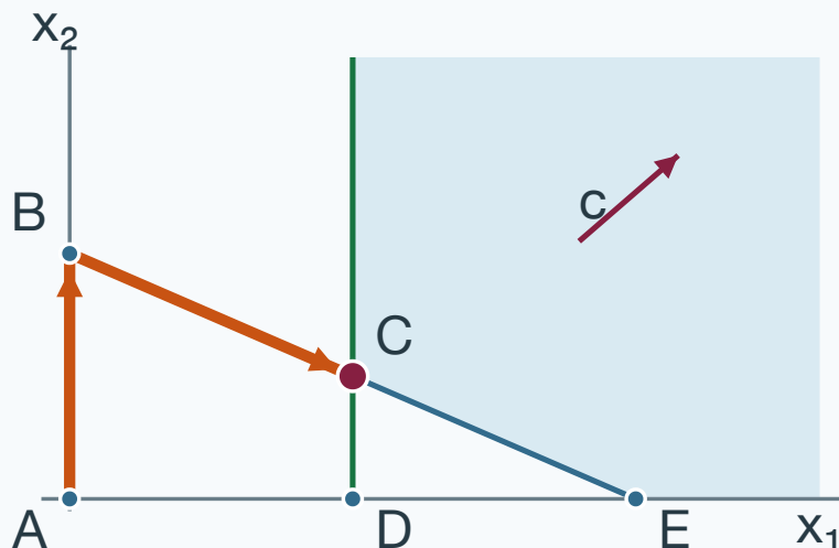
Primal variables
