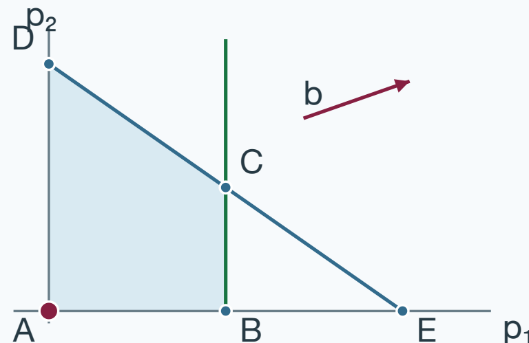
Dual variables
