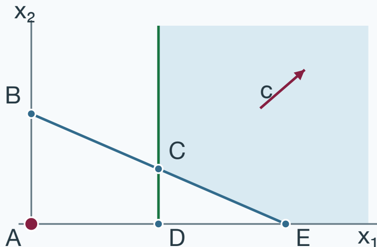
Primal variables
