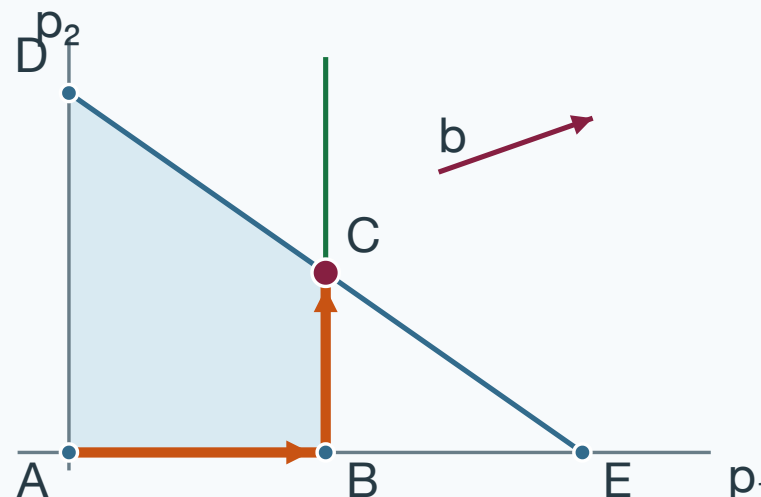
Dual variables
