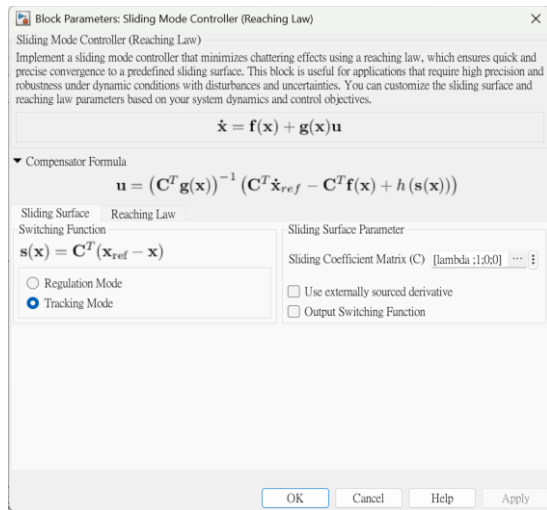
Fig. 2. SMC Controller in Simulink
