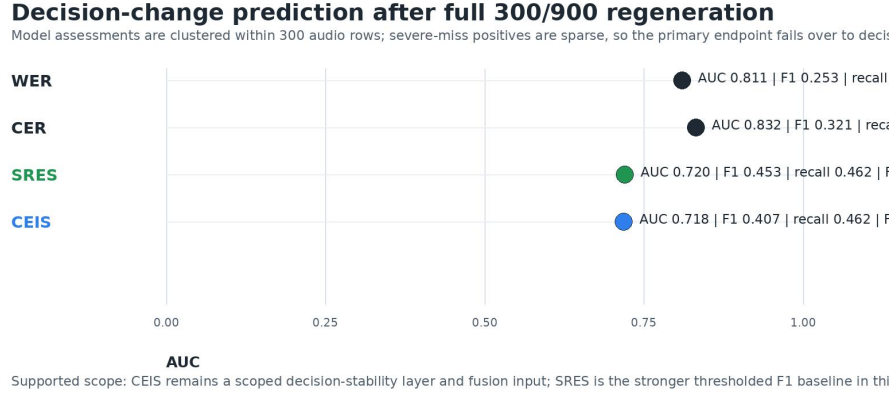
Figure 3: Final 300/900 regeneration evaluates decision-change prediction under clustered analysis; severe-miss replay is descriptive because row-level severe positives are sparse. Source: final_cs1_predictor_performance.tsv ; final_cs1_auc_delta_bootstrap.tsv ; final_cs1_residual_gain_after_sres.tsv .
