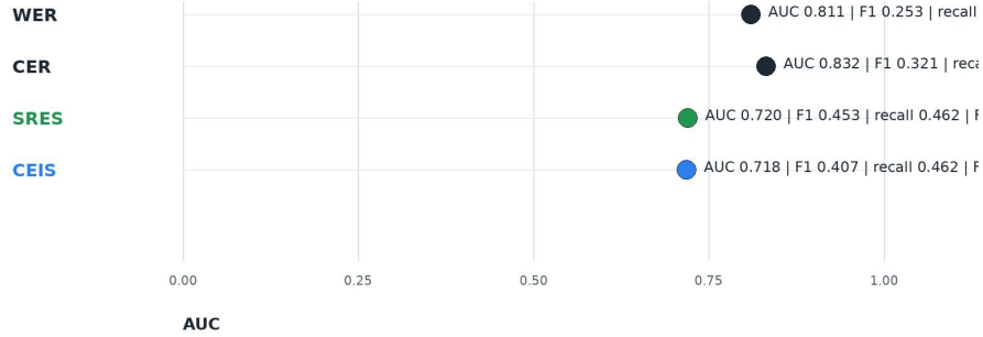
Figure 3: Final 300/900 regeneration evaluates decision-change prediction under clustered analysis; severe-miss replay is descriptive because row-level severe positives are sparse. Source: final_csl_predictor_performance.tsv ; final_csl_auc_delta_bootstrap.tsv ; final_csl_residual_gain_after_sres.tsv .
