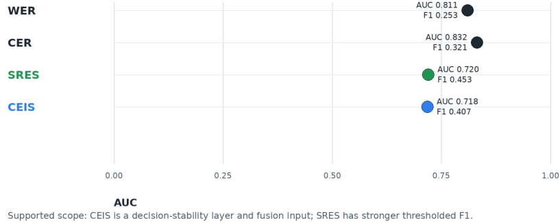
Figure 3: Final 300/900 regeneration evaluates decision-change prediction under clustered analysis; severe-miss replay is descriptive because row-level severe positives are sparse. Source: final_csl_predictor_performance.tsv ; final_csl_auc_delta_bootstrap.tsv ; final_csl_residual_gain_after_sres.tsv .
