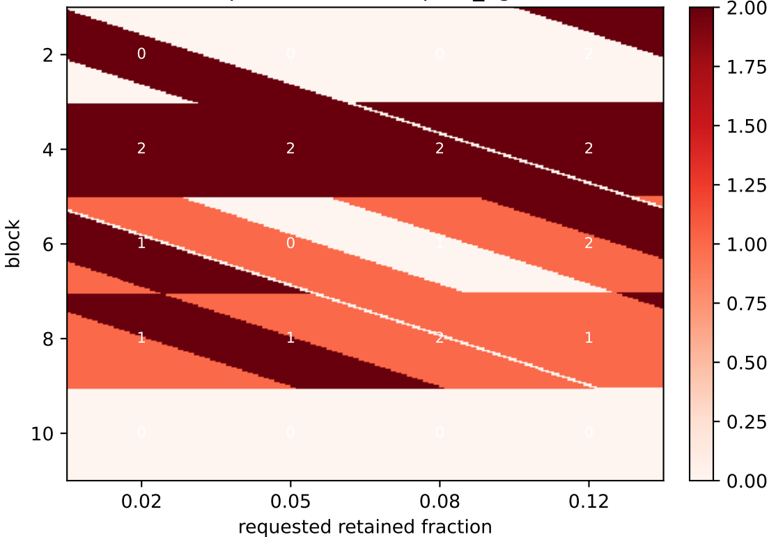
Collapse count (&lt; 0.5 pred_agree)
