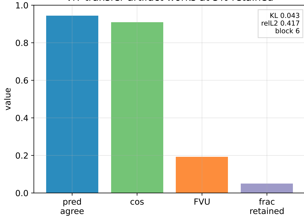
ViT transfer artifact works at 5% retained
