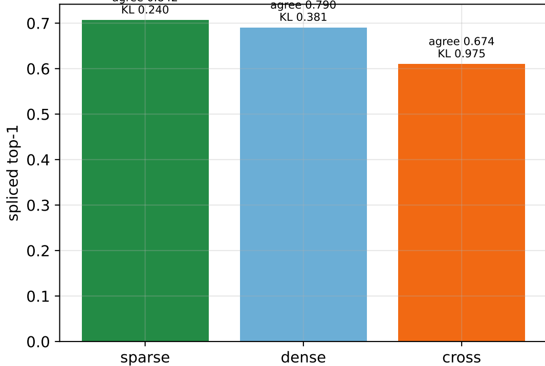
Q4→Q5 taxonomy: sparse is the best transition carrier
