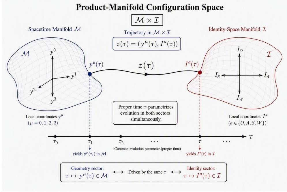
FIG. 2. Product-manifold configuration space \mathcal{M} \times \mathcal{I} . The trajectory z(\tau) = (y^\mu(\tau), I^a(\tau)) evolves simultaneously through the spacetime manifold \mathcal{M} and the identity-space manifold \mathcal{I} under a common proper-time parameter \tau .
