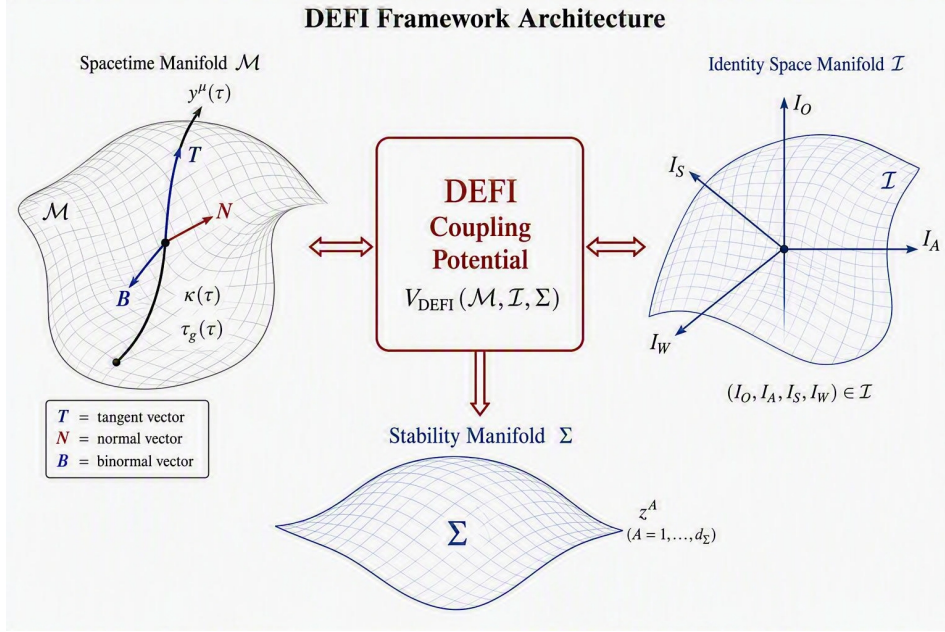
FIG. 1. Conceptual structure of DEFI as the variational bridge between SEFI identity-space dynamics and GWFM worldline geometry. The coupled DEFI framework generates the integrated consistency conditions that appear in the unified geometric field theory.
