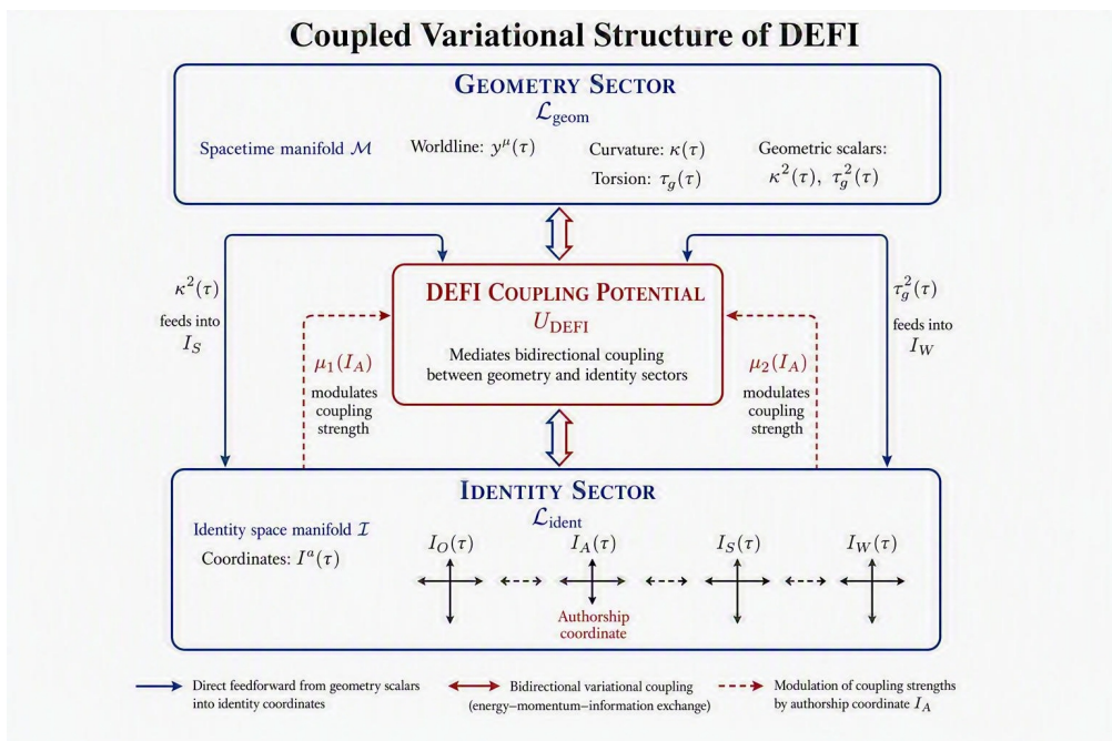
FIG. 3. Variational structure of DEFI. The coupling potential mediates bidirectional interaction between GWFM geometry variables and SEFI identity variables, with authorship-dependent coupling strengths.
