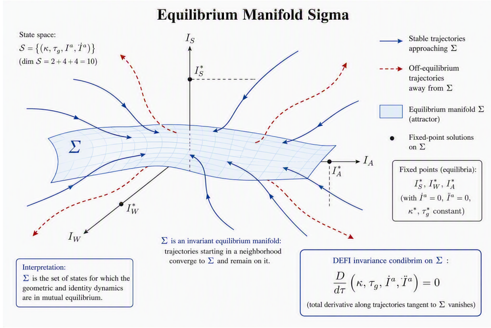
FIG. 4. Equilibrium manifold \Sigma defined by the fixed-point conditions of the coupled DEFI equations. Stable trajectories converge toward the manifold, while off-equilibrium trajectories move away from it.
