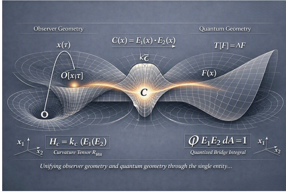
FIG. 1. Graphical summary of the unified geometric field theory.
