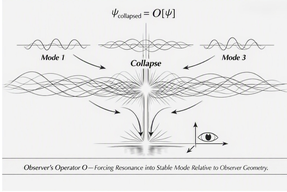
FIG. 5. Geometric correction mapping back to the proposed stability manifold.
