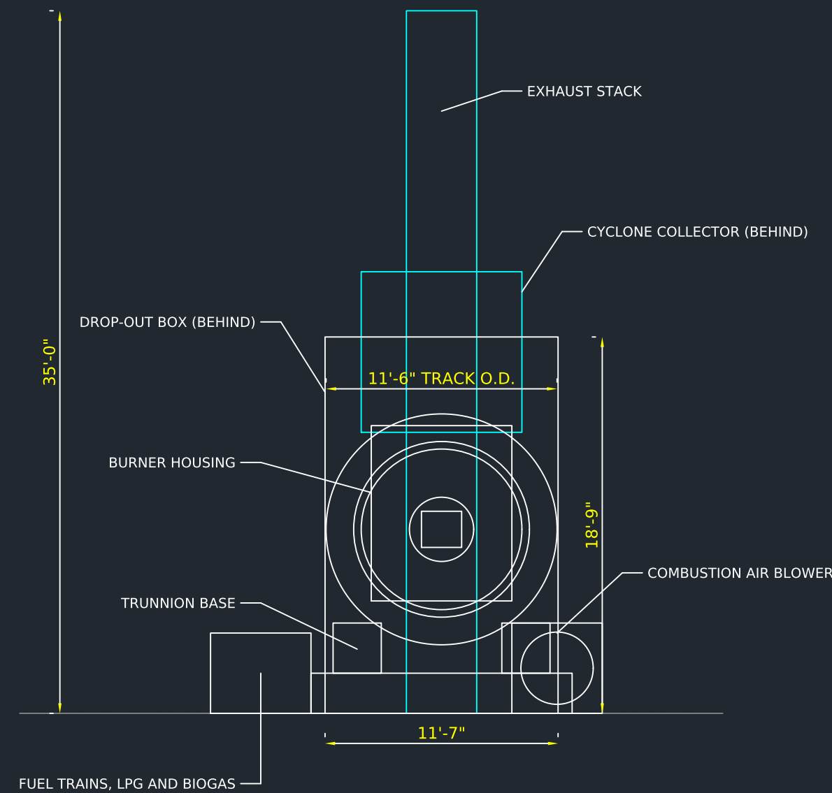
END VIEW
