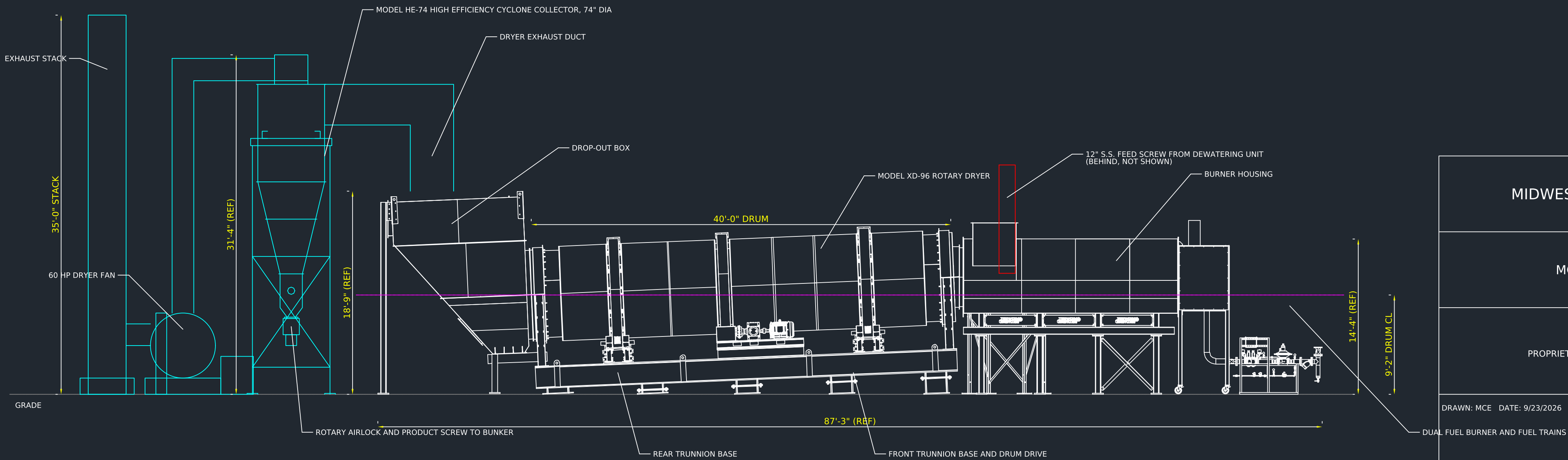
ELEVATION VIEW
