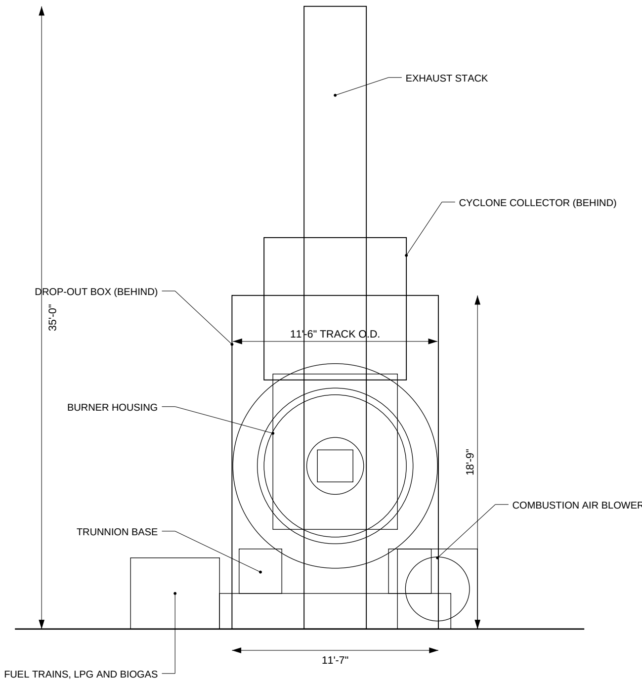
END VIEW MODEL XD-96 DRYER SYSTEM Scale 3/16" = 1'-0"
