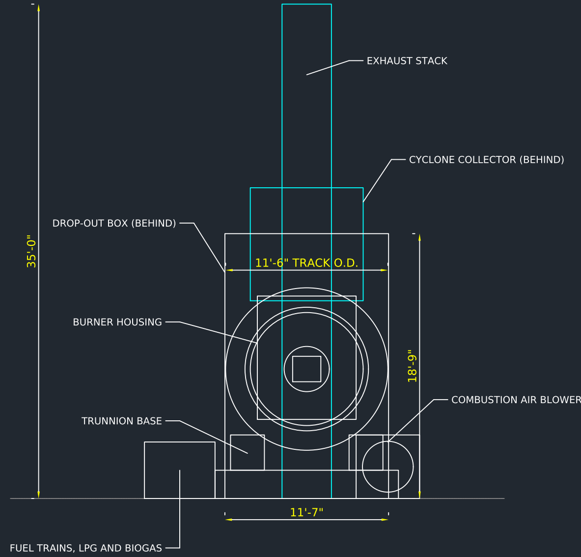
END VIEW
