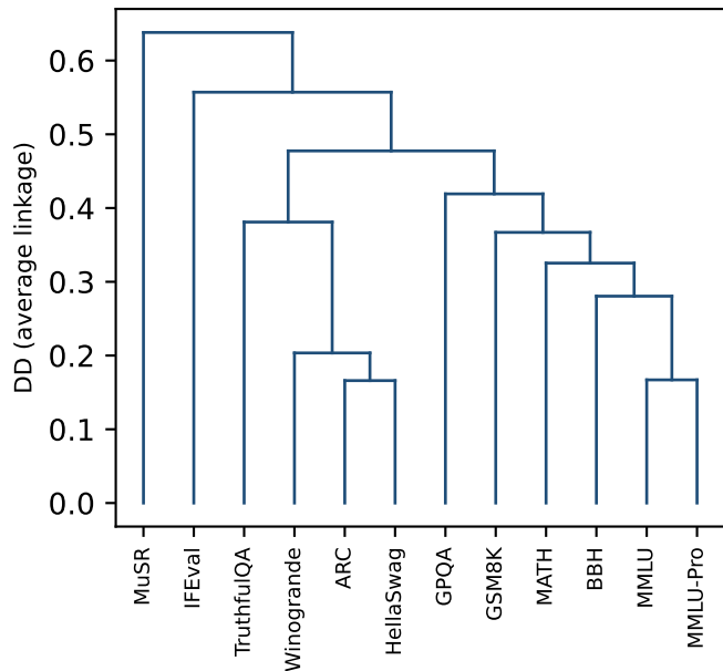
Benchmark clustering by DD distance
