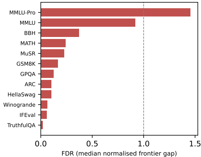
Frontier resolution per benchmark
