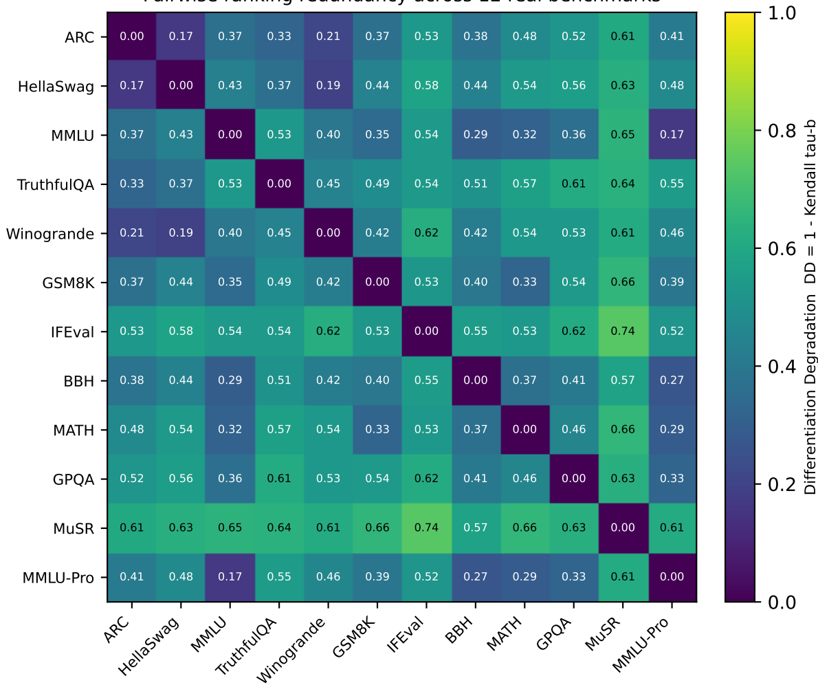
Pairwise ranking redundancy across 12 real benchmarks
