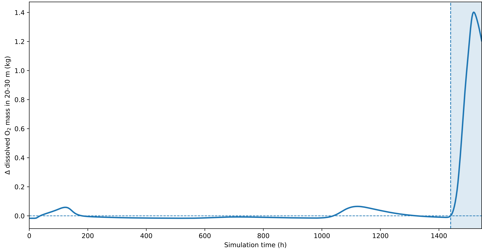
Deep O 2 inventory change relative to 1440 h
