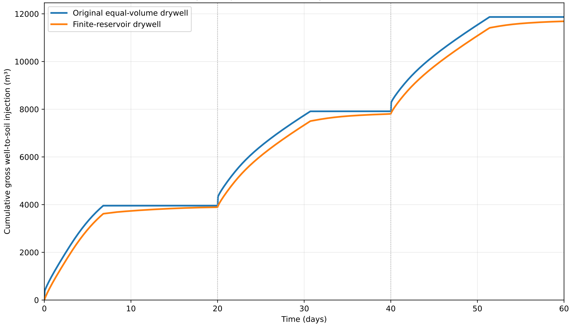
Drywell injection volume: original vs finite reservoir
