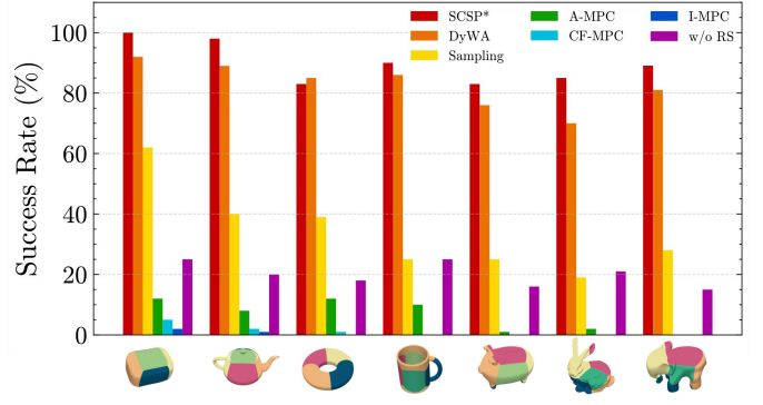
Fig. 8. Experimental results of robot manipulation in simulation. SCSP significantly outperforms other model-based methods and exceeds the performance of well-trained learning-based methods.
