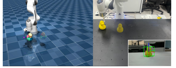
Fig. 11. Perception method in the real-world experimental setting. Object pose is detected using FoundationPose and filtered via a Kalman filter. Contact estimation is performed using a MuJoCo implementation that approximates the experimental environment.
