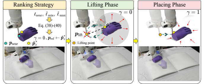
Fig. 6. Illustration of the CPO-based contact planning module. (a) Ranking strategy. When \mathbf{p}_{\text{near}} is evaluated infeasible, \gamma turns to zero and \mathbf{p}_{\text{ref}} \leftarrow \hat{\mathbf{p}}_r^* . The evaluation runs continuously in real-time. (b) When \gamma = 0 , the robot is guided by the potential field to \mathbf{p}_{\text{lift}} . (c) Once above \hat{\mathbf{p}}_r^* or the nearest point \mathbf{p}_{\text{ref}} to the robot is detected feasible via (30), \gamma becomes 1 and an attractive potential is applied, guiding the robot to contact with the object.
