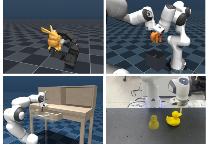
Fig. 1. SCSP enables online contact selection and closed-loop generation of diverse manipulation trajectories, allowing it to address a wide range of challenging contact-rich manipulation tasks.
