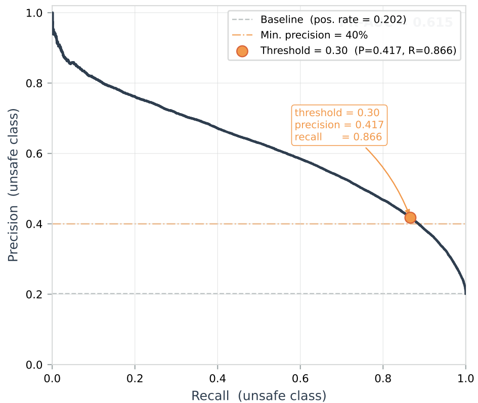
Precision-recall curve (test set)
