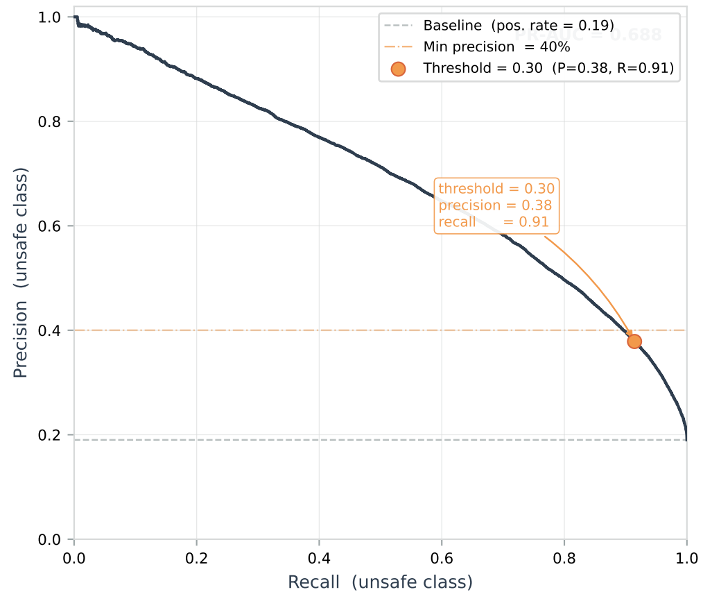
Precision-recall (test set)
