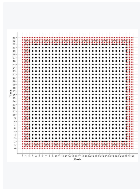
Fine-to-coarse grid interface from the meshing script.
