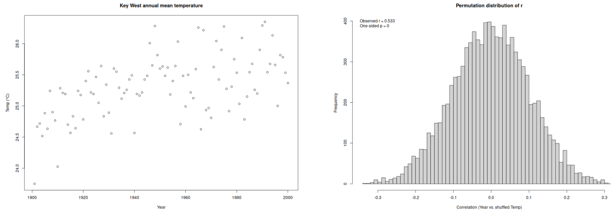
Figure 1: Left: Year vs. temperature. Right: permutation distribution (red line: observed r ).
