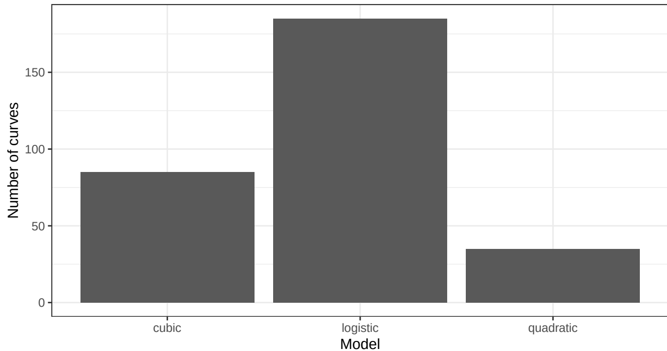
Model wins by AIC
