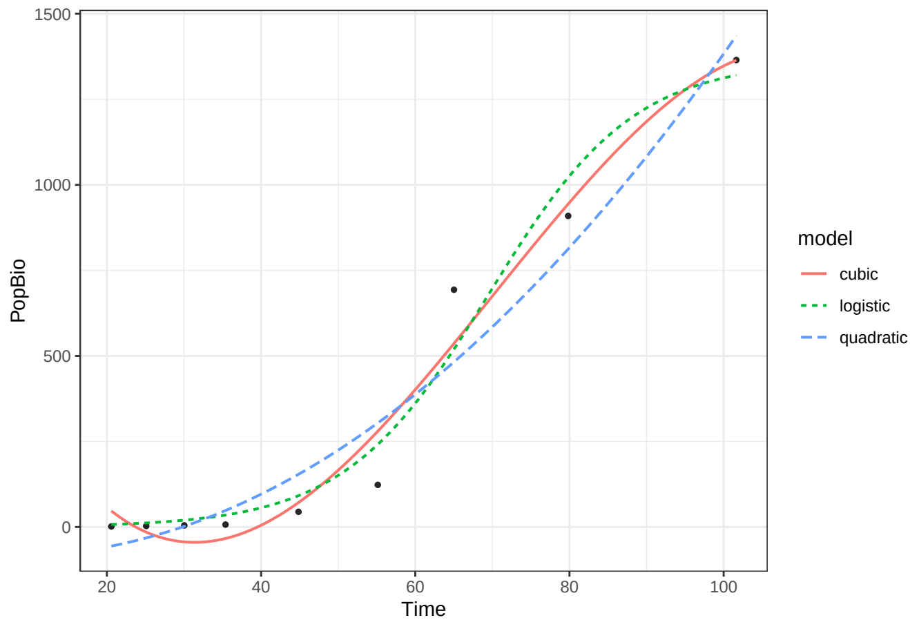
Curve 17 | Units: CFU | Temp: 15
