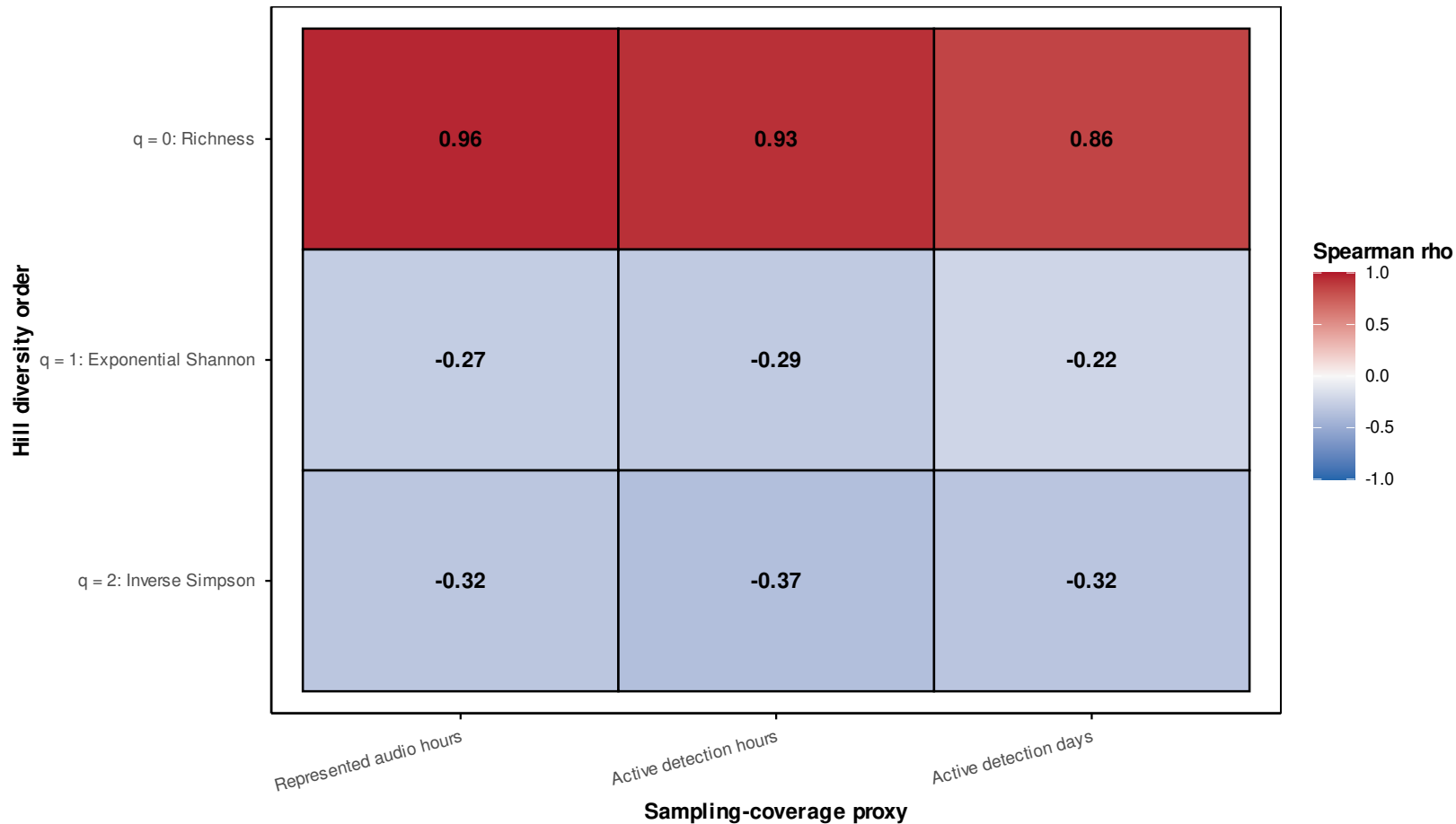
Spearman correlations between monthly diversity and coverage proxies
