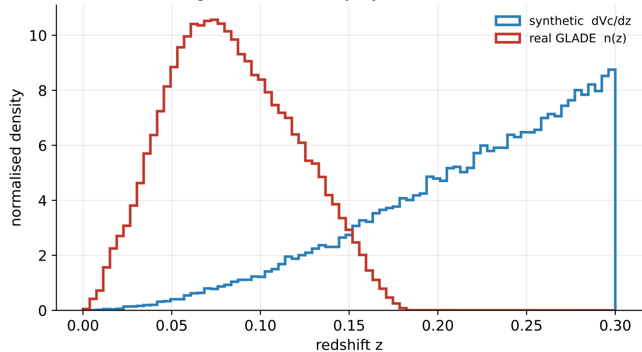
Catalogue redshift density: synthetic vs real GLADE
