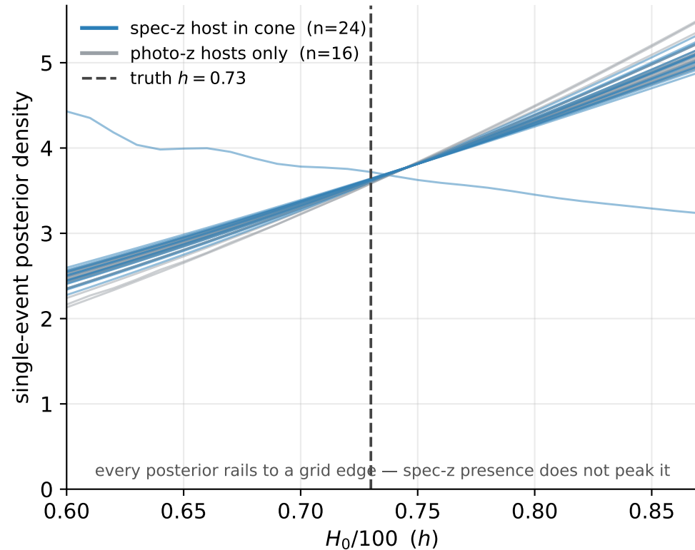
(A) single-event posteriors coloured by spec-z presence
