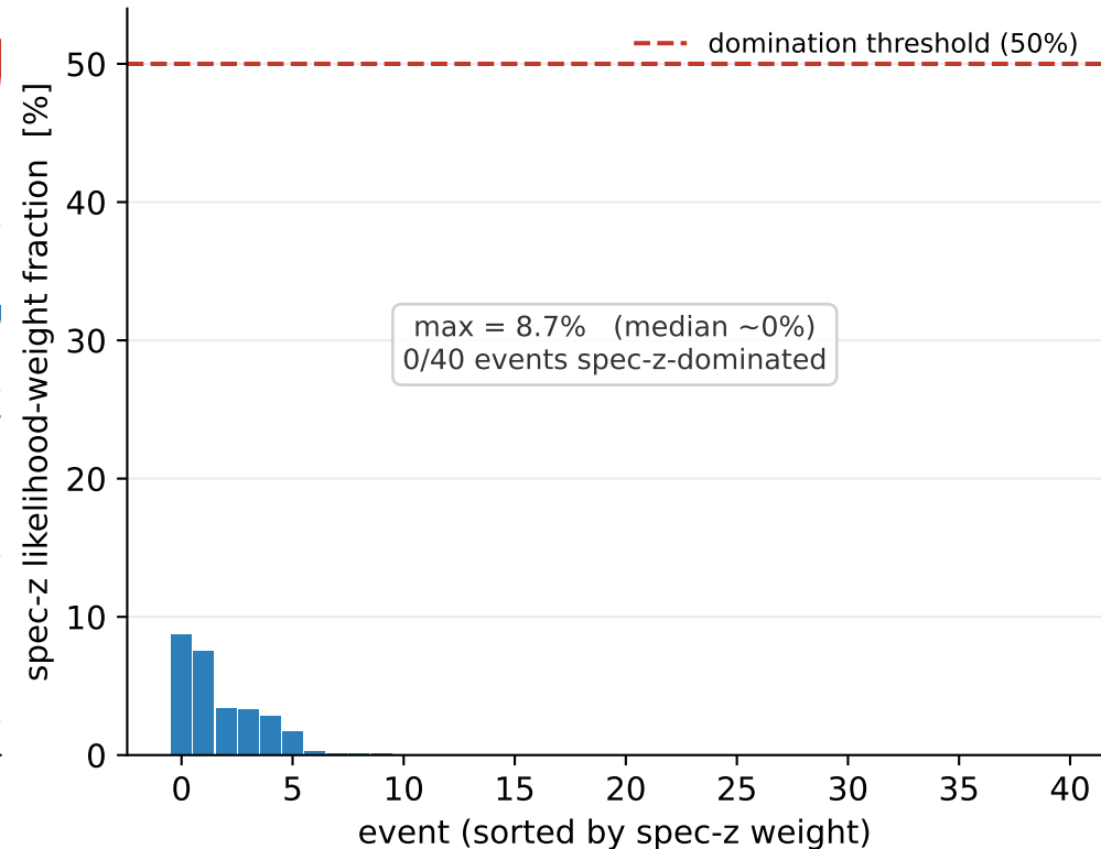
(C) spec-z weight per event (never reaches domination)
