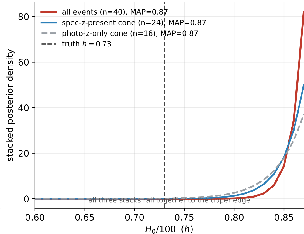
(B) stacked posterior, spec-z / photo-z decomposition
