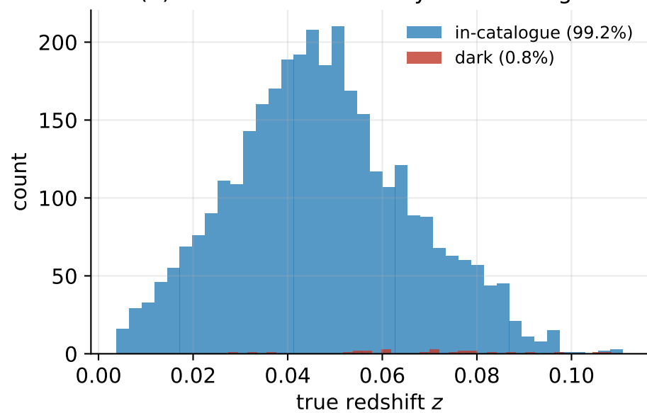
(d) detections are nearby & in-catalogue
