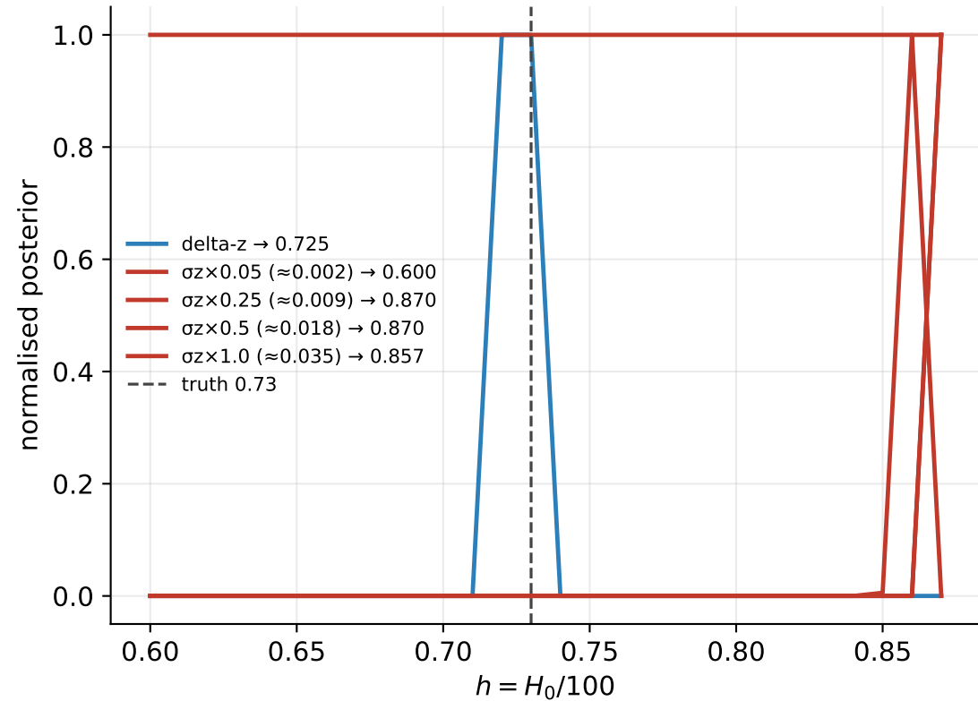
(a) catalogue photo-z error rails the inference
