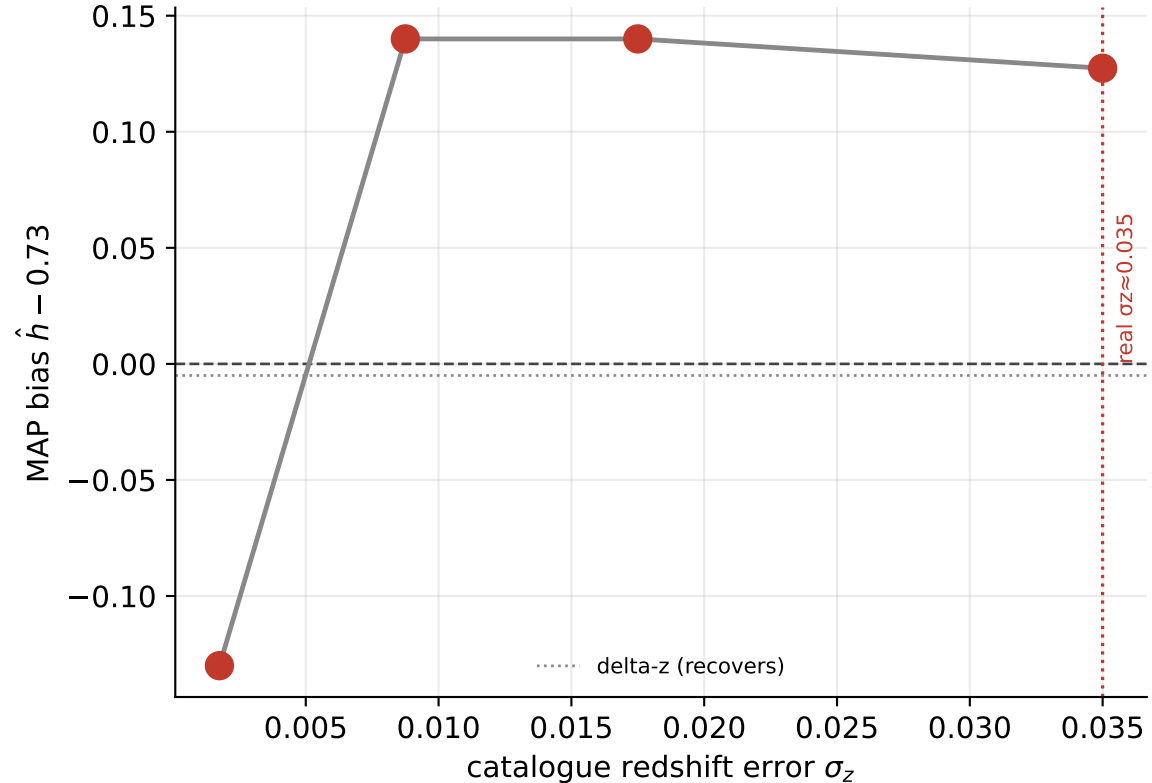
(b) bias vs photo-z error (the fix: small \sigma_z )
