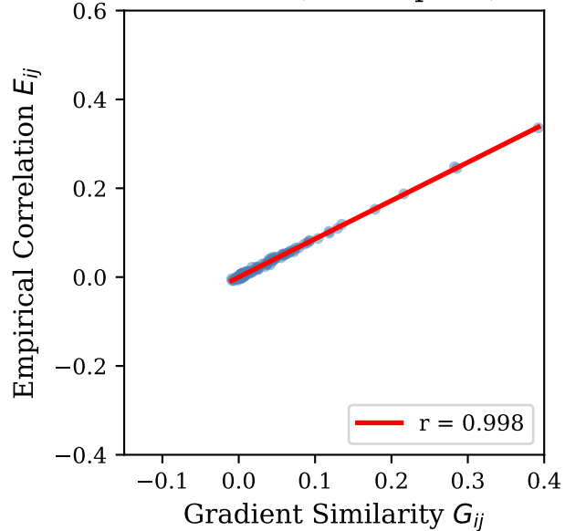
ToxCast (n=136 pairs)
