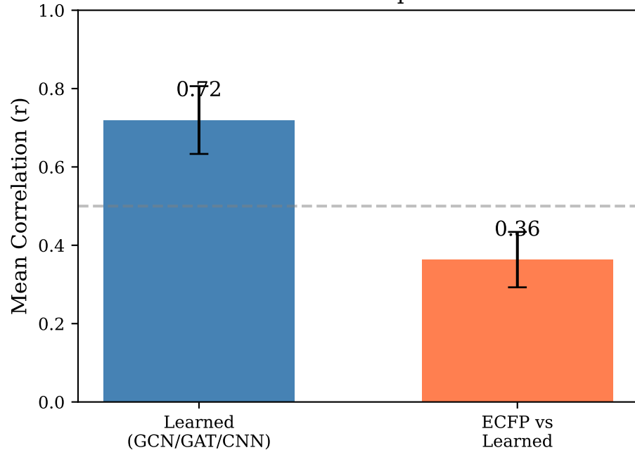
Learned vs Fixed Representations
