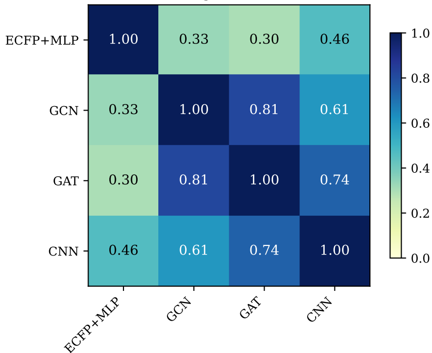
Architecture Agreement (Pearson r)
