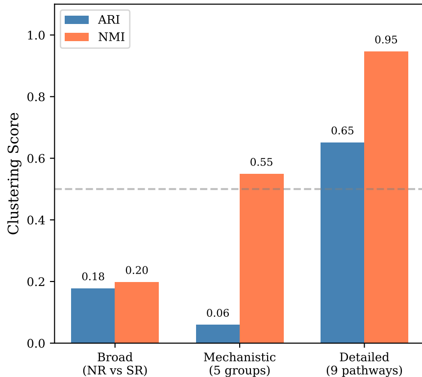
Pathway Recovery Performance
