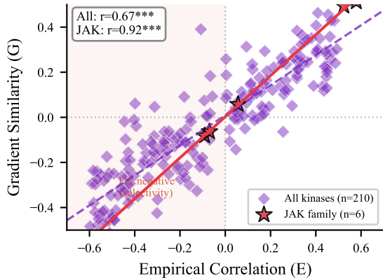
A. Kinase Selectivity Validation
