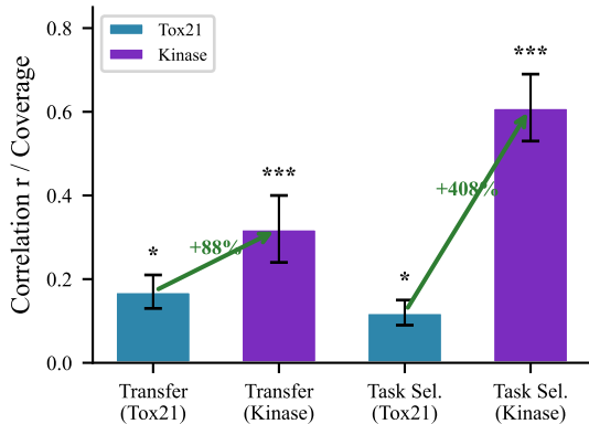
B. Kinase vs Tox21 Applications
