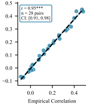
A. Within-Toxicity
