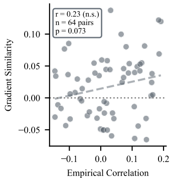
C. Cross-Domain
