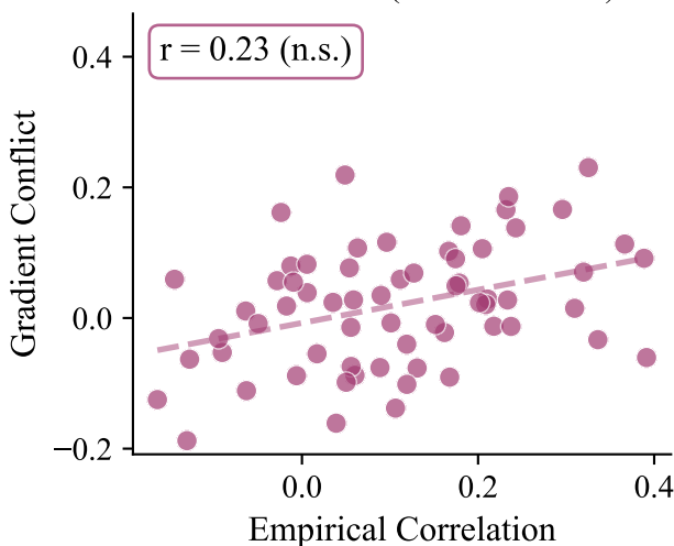
B. Cross-Domain (Tox vs ADME)
