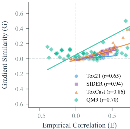
A. Gradient vs Empirical Correlation
