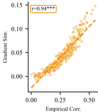
D. SIDER (100%)
