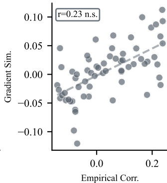
B. Cross-Domain
