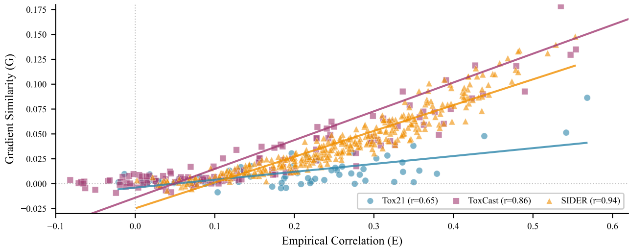
A. Gradient Similarity vs Empirical Correlation Across All Datasets
