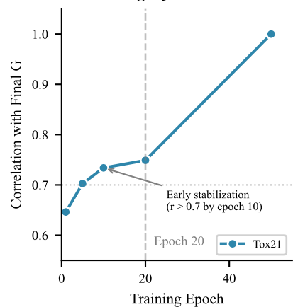
D. Training Dynamics
