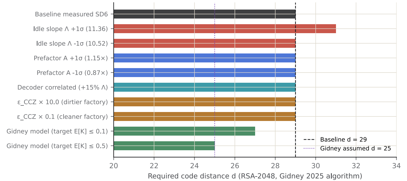
Tornado chart showing required code distance d for RSA-2048 (Gidney 2025 algorithm) across physical noise parameters, factory quality, decoder performance, and assumed models.
