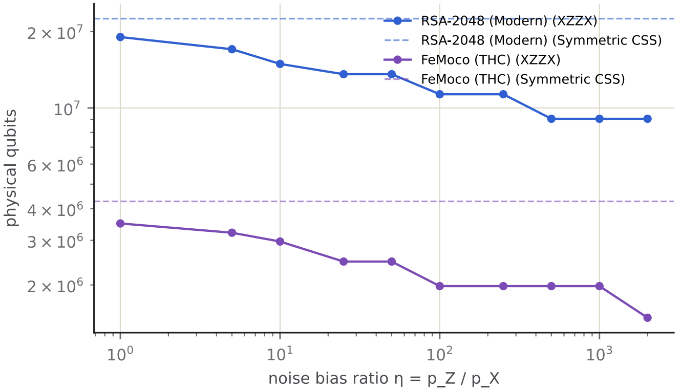
Physical qubit footprint as a function of noise bias ratio \eta = p_Z / p_X for RSA-2048 (modern arithmetic) and FeMoco (THC) under asymmetric XZZX surface codes, compared against symmetric CSS baselines.
