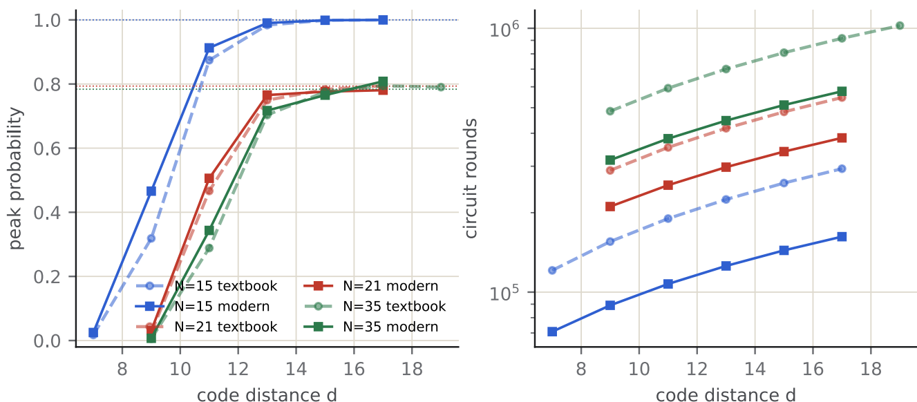
Modern vs. textbook Shor on the simulated machine (cultivated magic states, p = 0.1\% ). Left: peak probability vs. distance d . Right: total circuit execution rounds.
