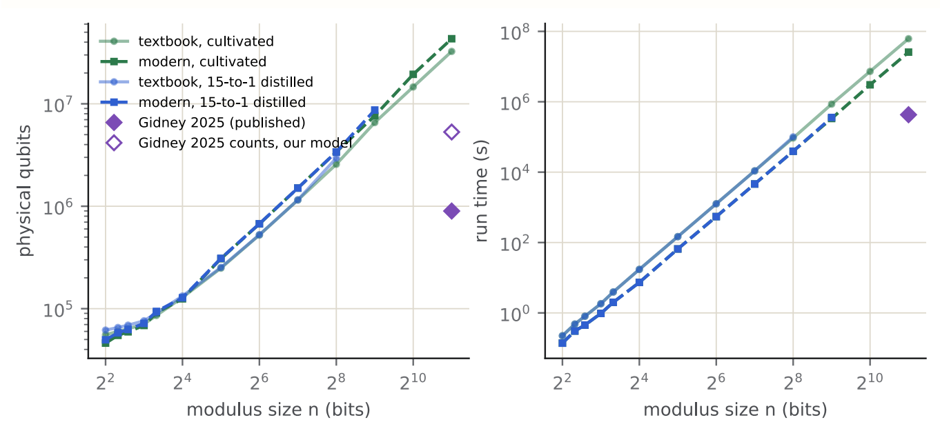
Shor scaling from the simulated sizes to RSA-2048 ( p = 0.1\% ). Modern windowed arithmetic cuts runtime across all sizes.
