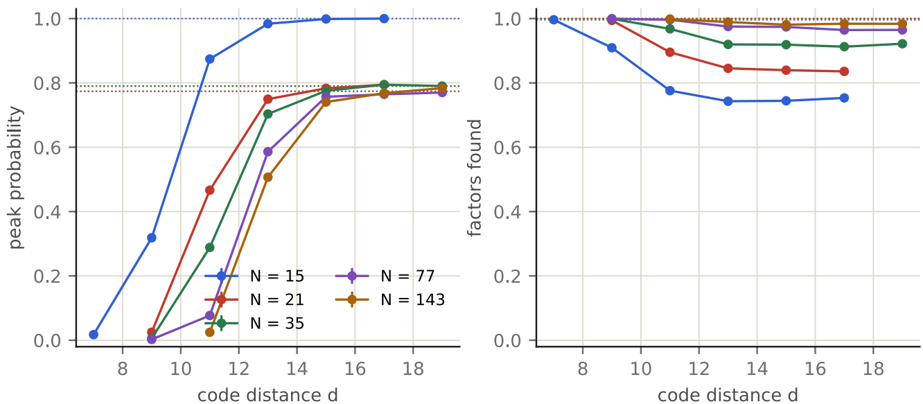
Left: peak probability vs d (cultivated states, p = 0.1\% ); dotted: noiseless. Right: the same runs scored by factors found; dotted: random-outcome baseline.
