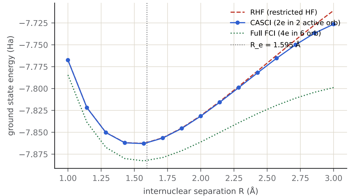
LiH potential energy dissociation curve comparing Restricted Hartree-Fock (RHF), CASCI(2, 2) with frozen 1s^2 core, and full 4-electron FCI in STO-3G. The equilibrium geometry R_e = 1.595 Å is marked with a vertical dotted line.
