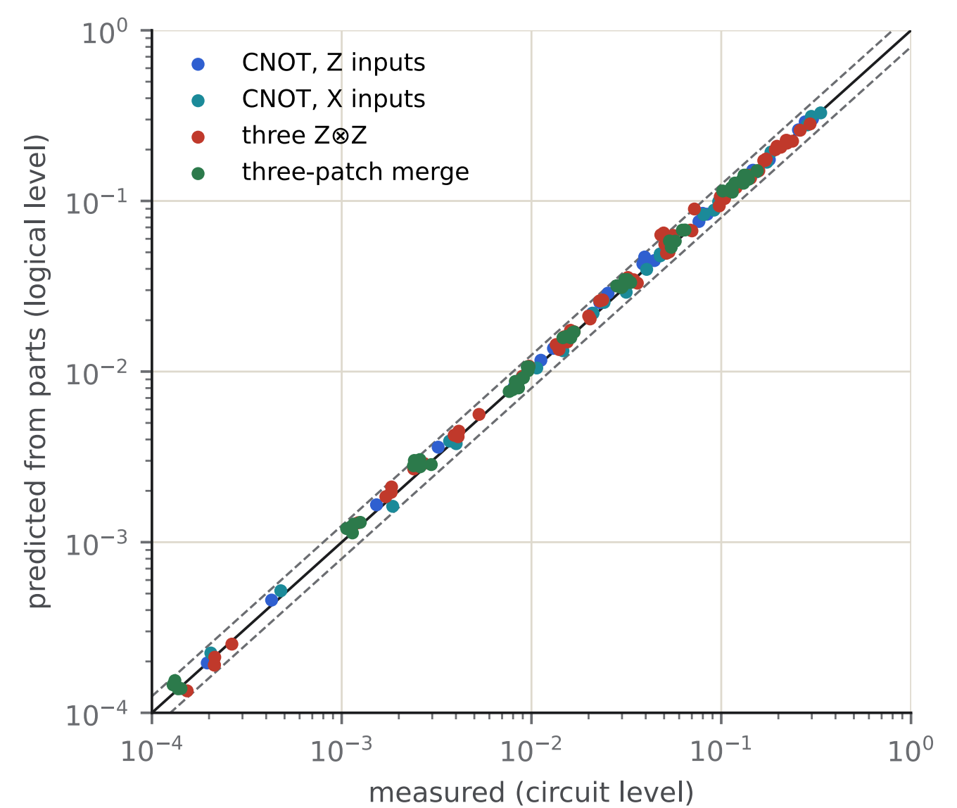
Observable failure rates of whole surgery experiments: predicted from calibrated parts by ftsim vs measured at circuit level; dashed \pm 25\% .
