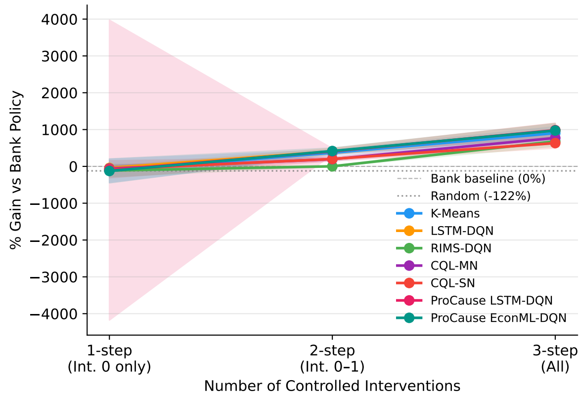
RCT Data
