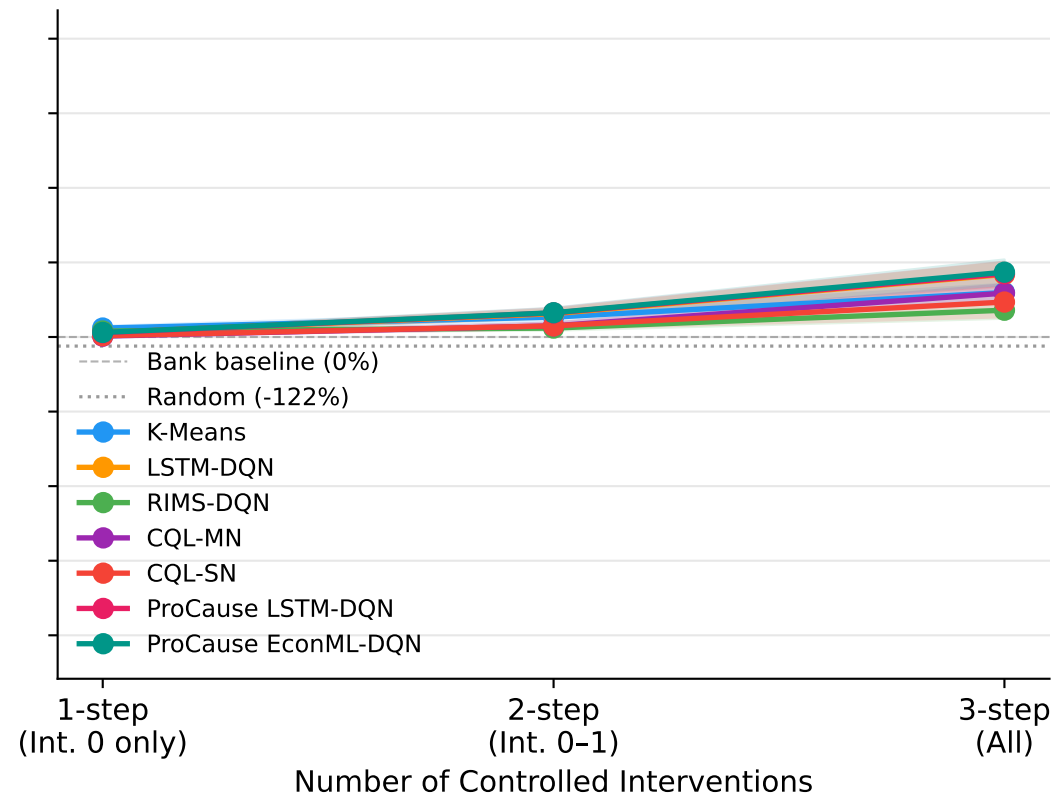
CONF Data
