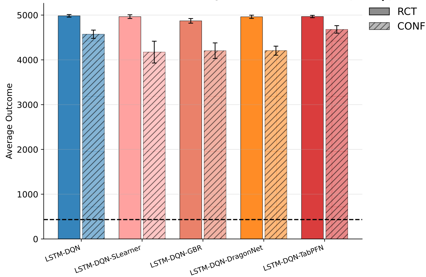
Causal Reward Estimation: LSTM-DQN Baseline vs Variants (3-step)
