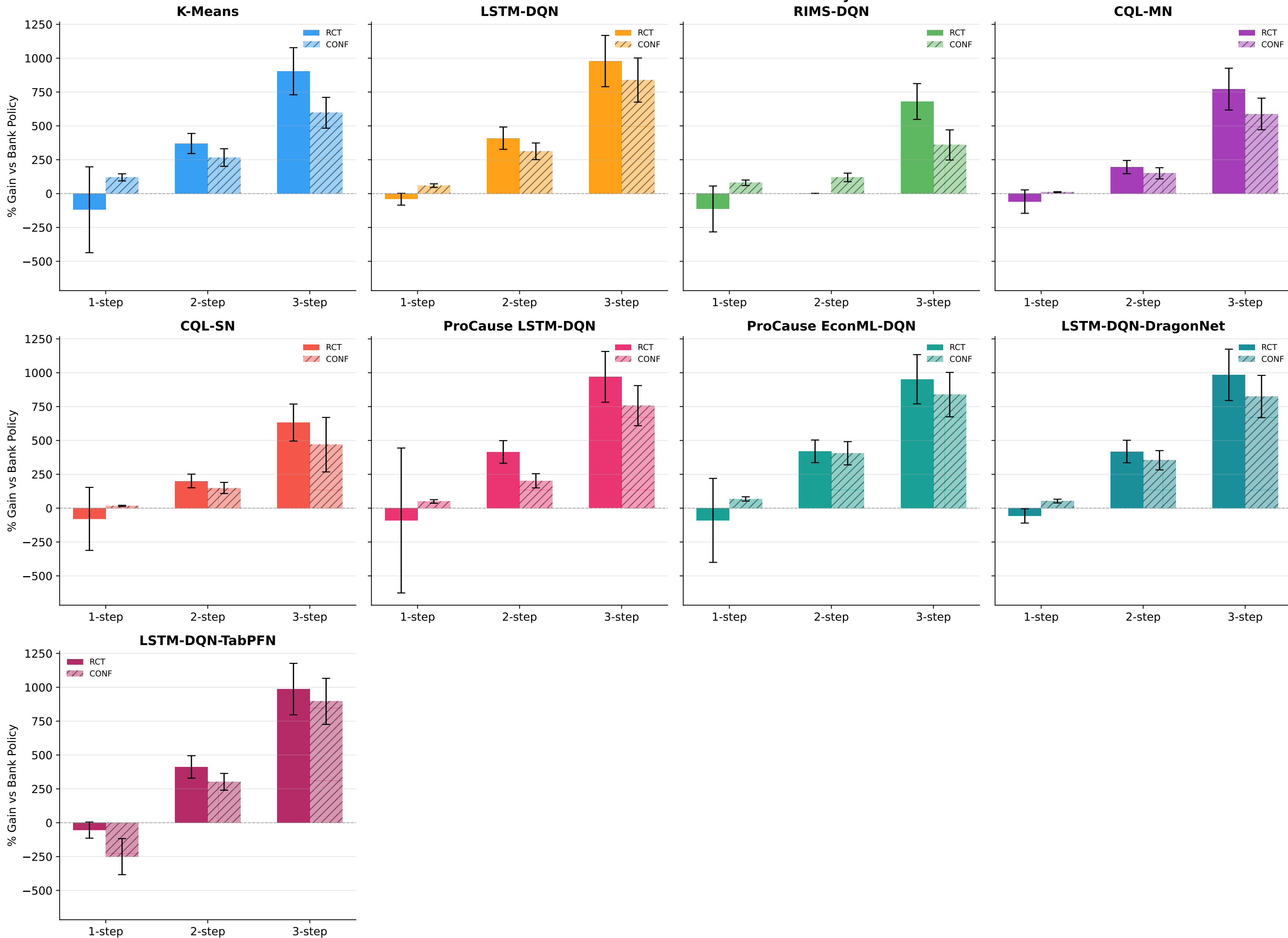
RCT vs. Confounded Data: % Gain over Bank Policy
