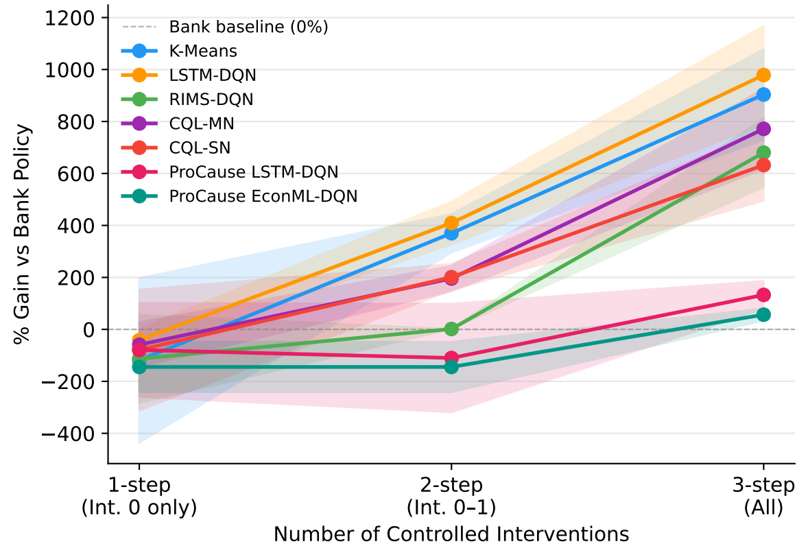
RCT Data
