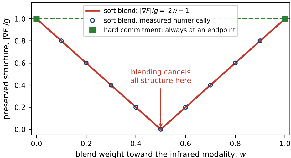
A soft weight cannot preserve a conflicting boundary
